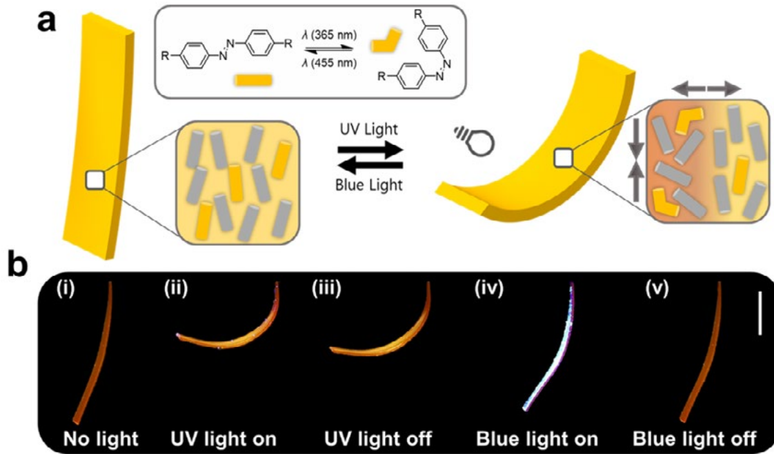
Mechanism and reversible bending behavior of the photoresponsive material
