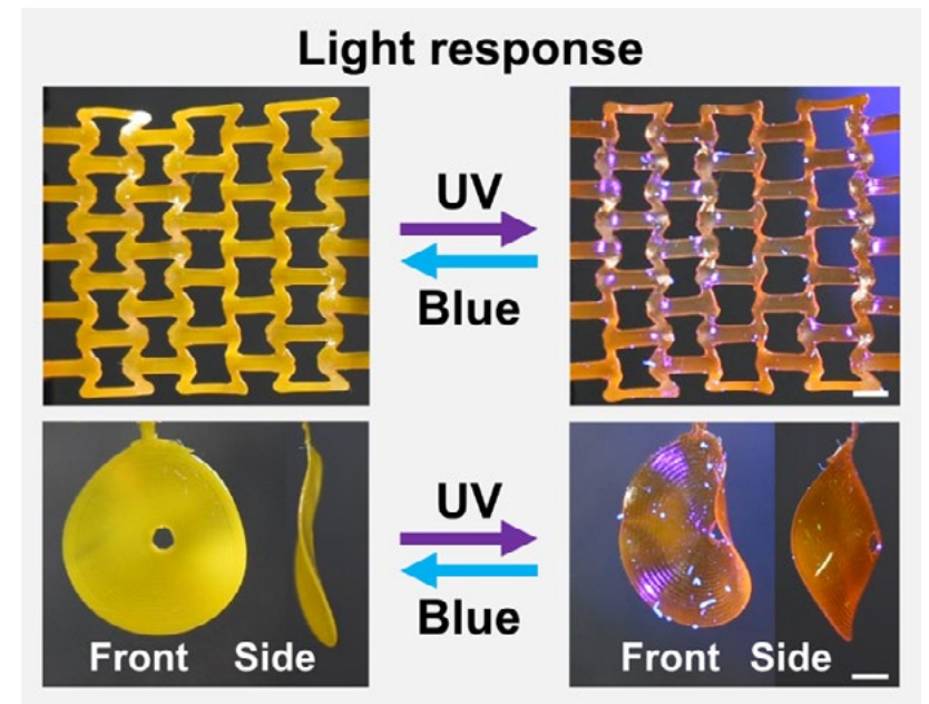
Reversible actuation of re-entrant honeycomb and spiral director structures
